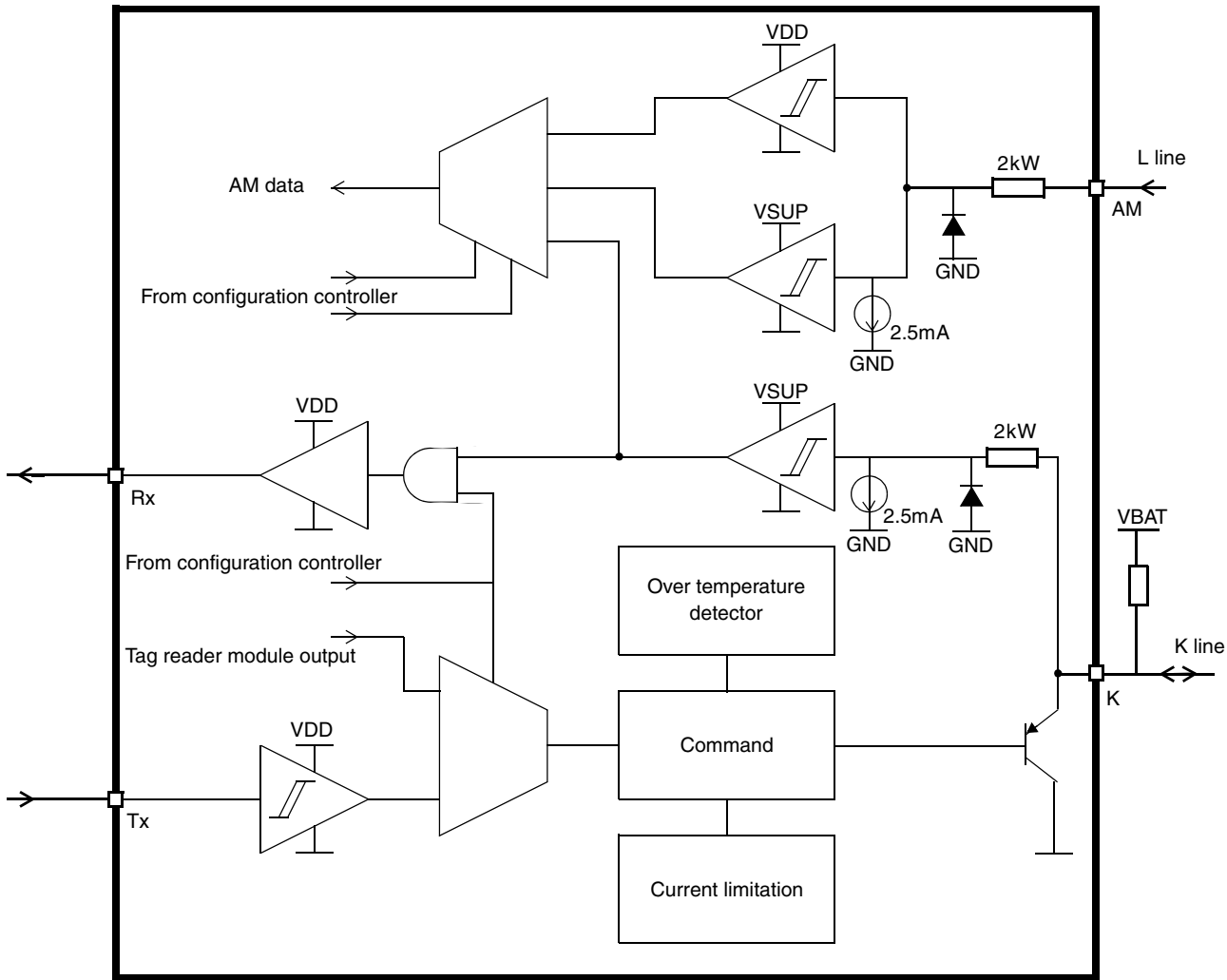
Figure 5. ISO 9141 Interface
