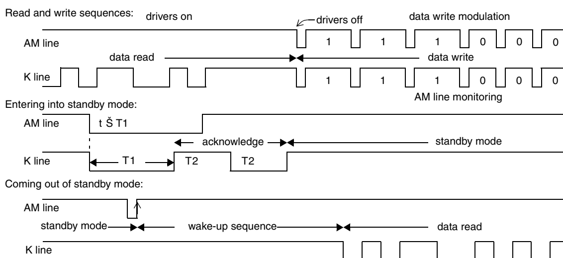
Figure 8. Modes Access Description in Two-wire Bus Configuration
