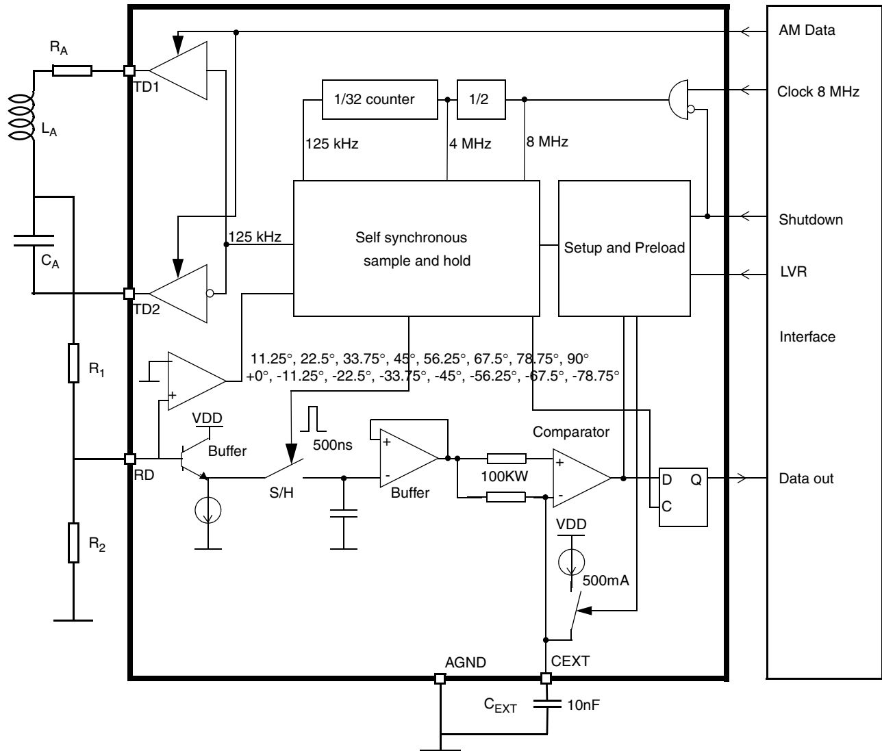
Figure 2. Tag Reader Block Diagram
