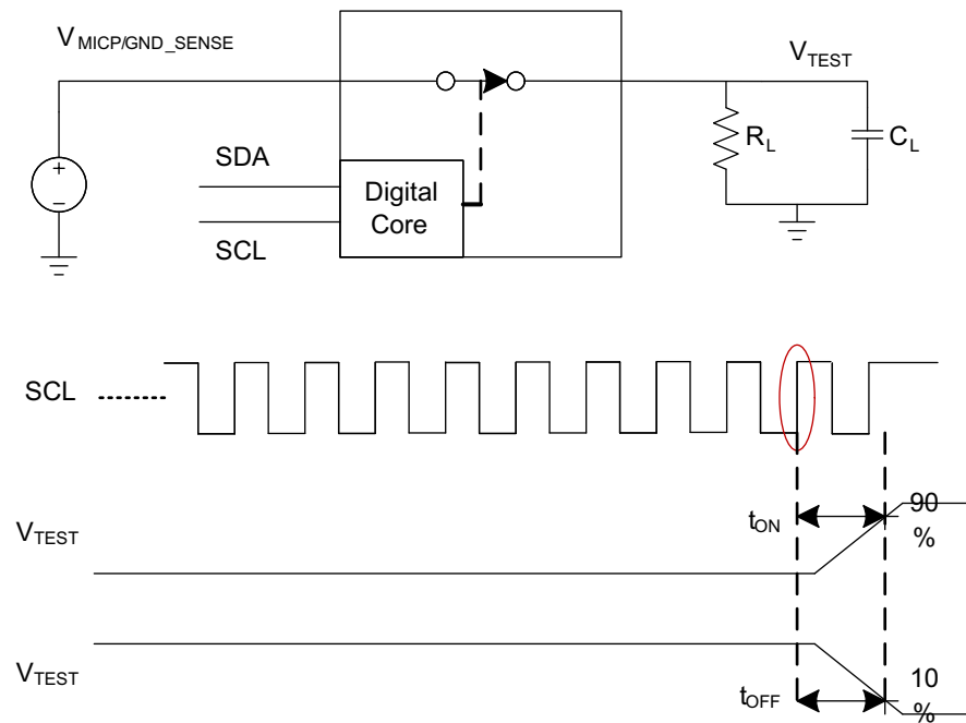
Figure 15. S3 t_{OFF}/t_{ON}
