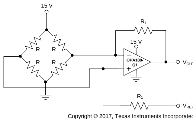
Figure 46. Bridge Amplifier
