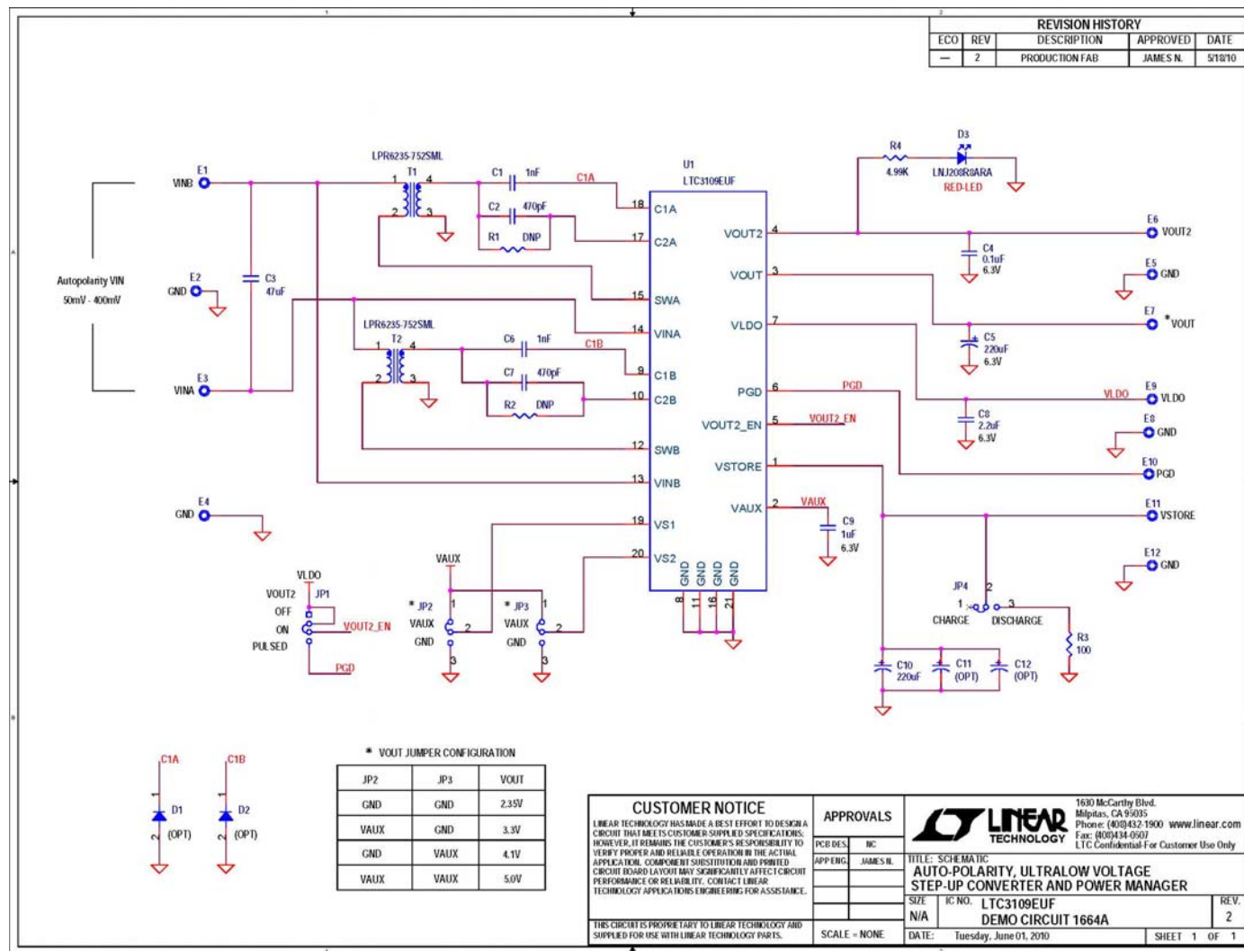
Figure 3. Circuit Schematic
