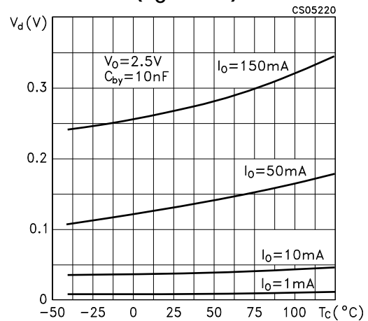
Figure 4. Dropout voltage vs. temperature ( V_O = 2.5\text{ V} )
