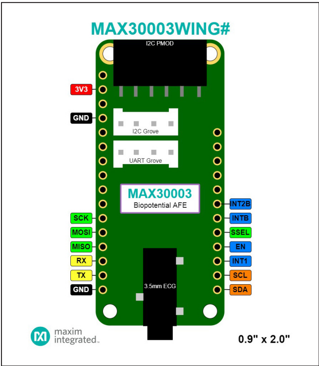
Figure 1. DIP Pinout
