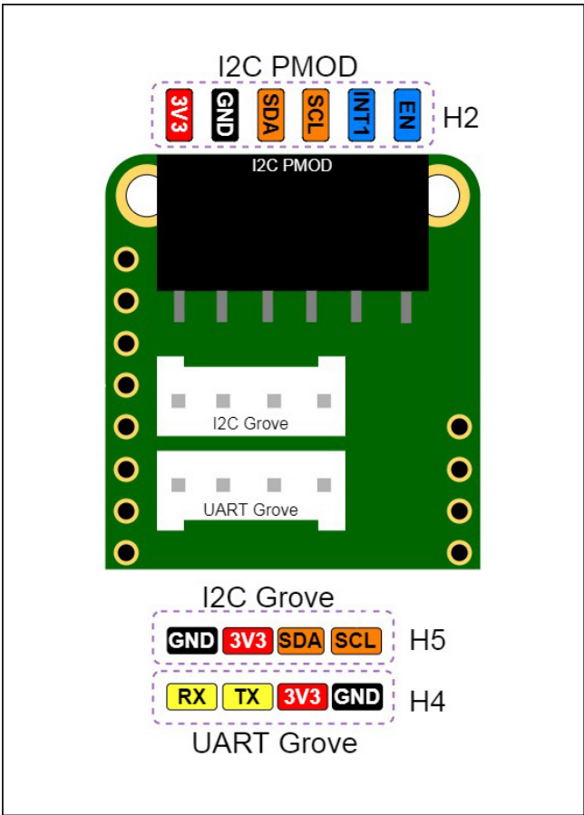
Figure 2. PMOD/Grove Connectors
