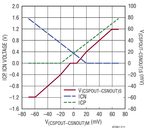
Figure 11. I_{OUT(SLAVE)} Control Voltage Relationships (CCM)
