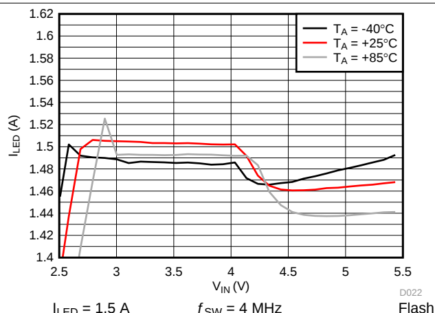
Figure 11. LED2 Current vs Input Voltage
