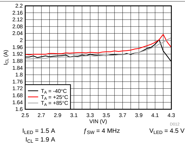
Figure 27. Inductor Current Limit vs Input Voltage
