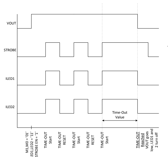
Figure 34. IR Mode Timeout
