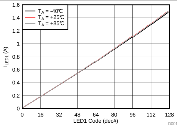
Figure 2. LED1 Flash Current vs Brightness Code
