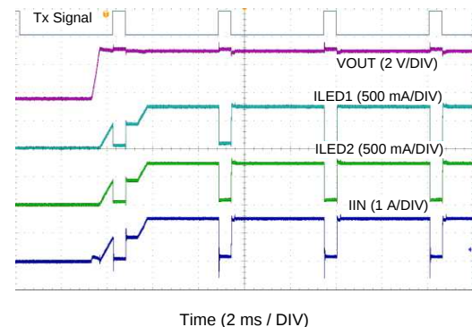
Figure 55. Start-Up
