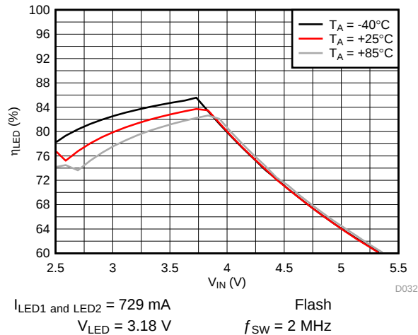
Figure 48. LED Efficiency vs Input Voltage
