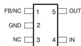
DCK PACKAGE SC70-5 (TOP VIEW)
