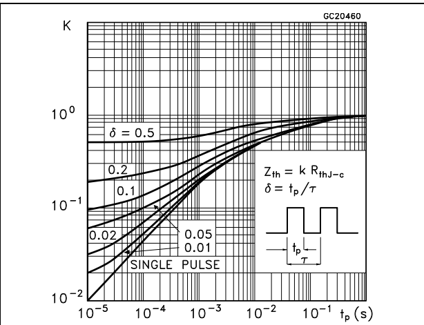
Figure 3. Thermal impedance for IPAK, DPAK
