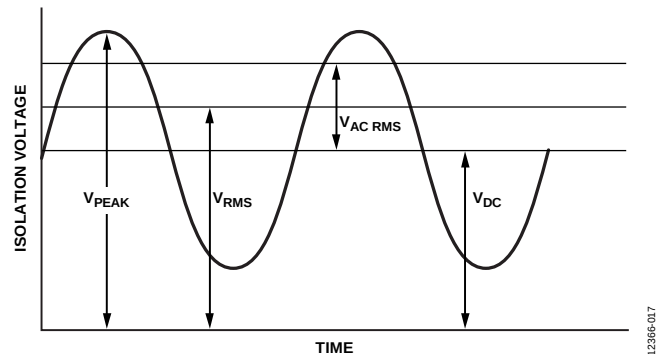
Figure 17. Critical Voltage Example
