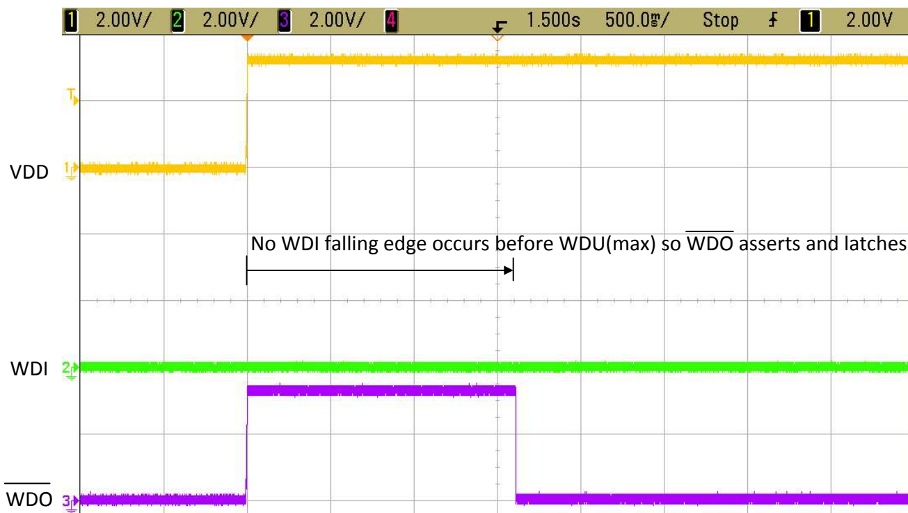
Figure 22. Watchdog Fault Caused by Missing WDI Pulse Shows \overline{\text{WDO}} Latching
