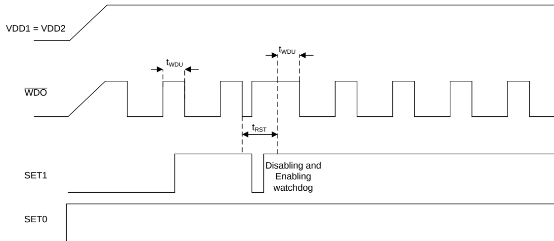
Figure 10. Enabling and Disabling the Watchdog Timer During a WDO Reset Event
