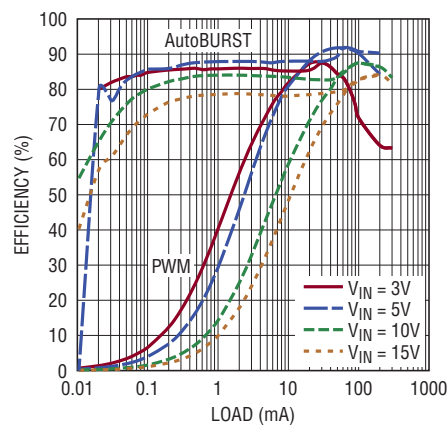
Figure 1. DC1923A Efficiency
