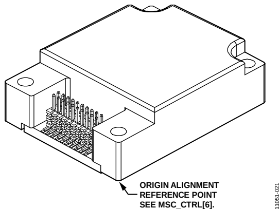
Figure 21. Point of Percussion Physical Reference
