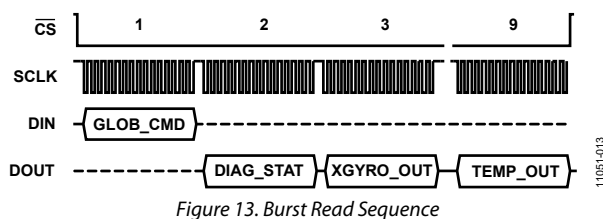
Figure 13. Burst Read Sequence
