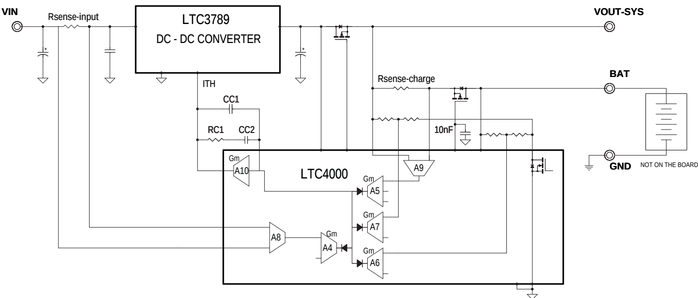
Figure 4. Block Diagram
