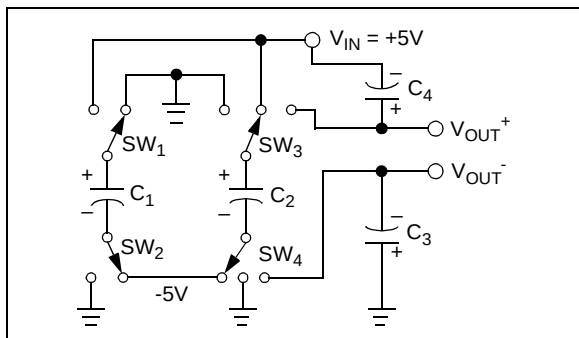
FIGURE 4-1: Charge Pump - Phase 1.
