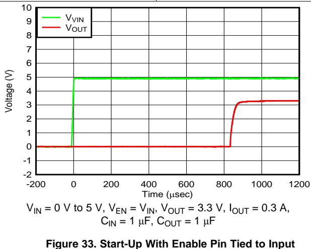
Figure 33. Start-Up With Enable Pin Tied to Input
