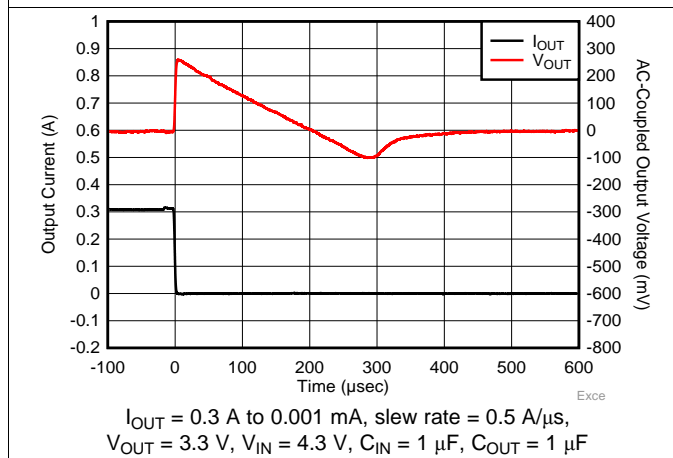
Figure 29. Load Transient
