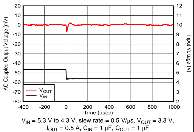
Figure 30. Line Transient
