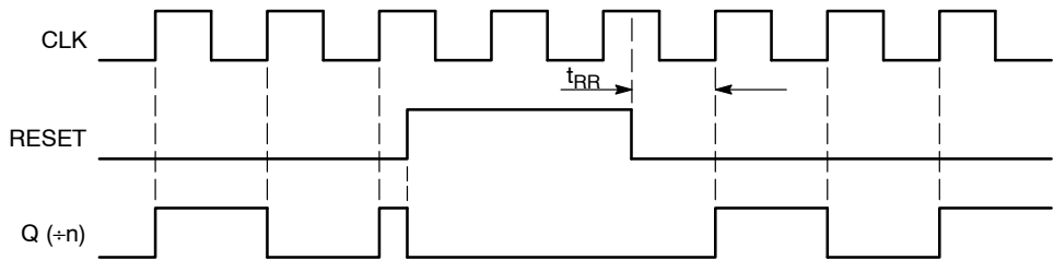
Figure 5. Timing Diagram
