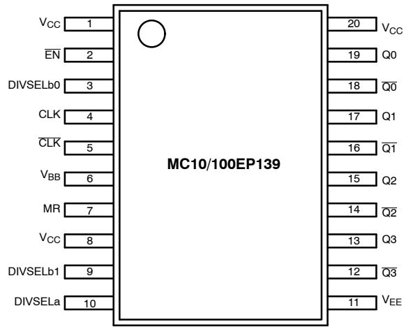
Figure 1. 20-Lead Pinout (Top View)
