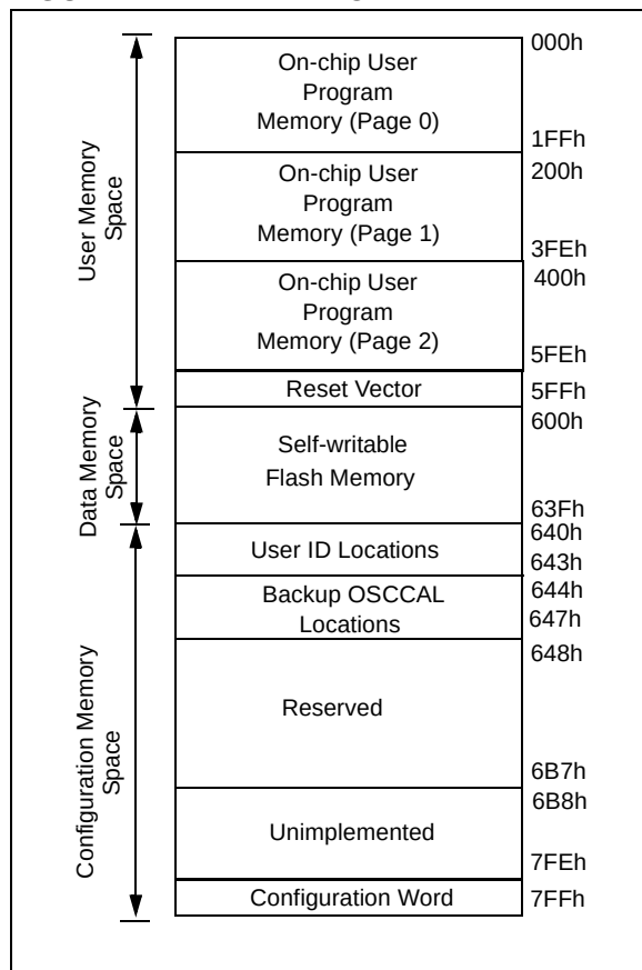
FIGURE 2-1: MEMORY MAP
