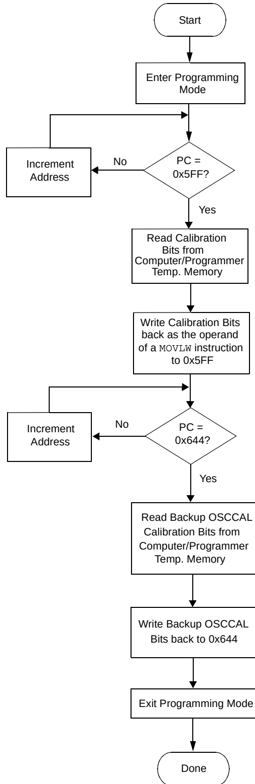
FIGURE 3-11: RESTORING/PROGRAMMING THE OSCCAL CALIBRATION BITS
