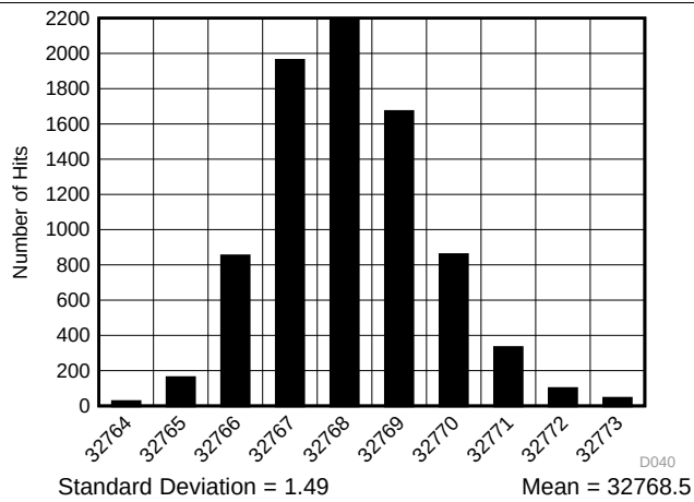
Figure 34. Typical DC Code Spread in High Precision Mode
