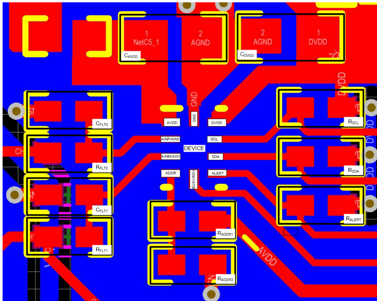
Figure 124. Example Layout
