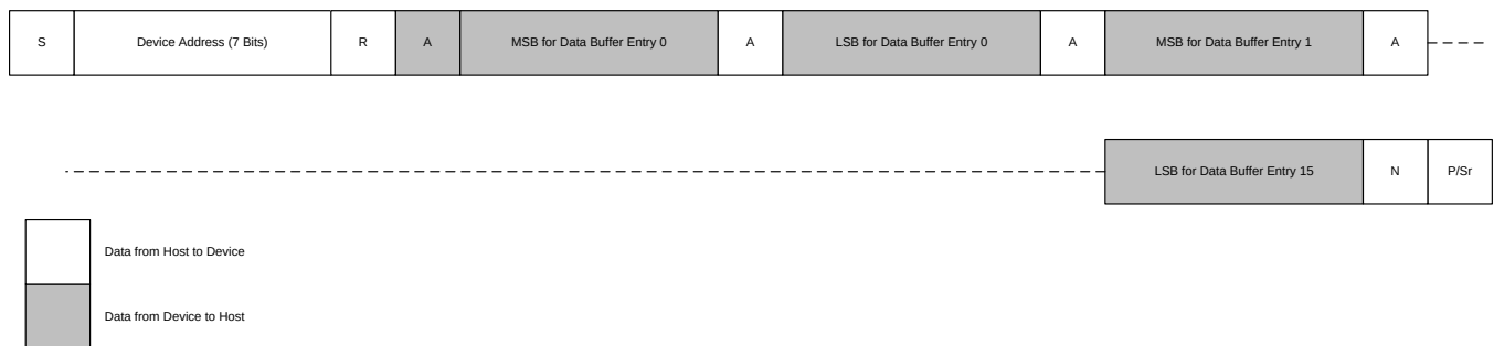
Figure 46. Reading Data Buffer (16 Bit Words × 16 Words)
