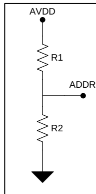
Figure 45. External Resistor Connection Diagram for ADDR Pin
