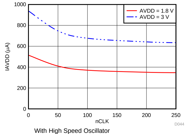
Figure 74. I_{AVDD} in High Precision Mode with nCLK
