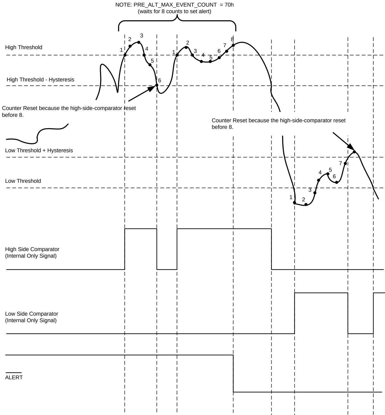
Figure 48. Thresholds, Hysteresis and Event Counter for Digital Window Comparator
