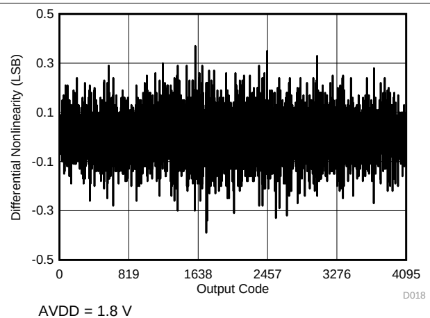
Figure 18. Typical DNL in Manual Mode
