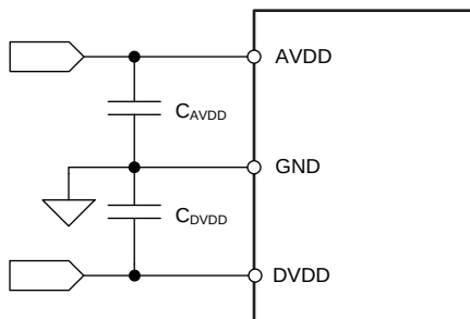
Figure 122. Power-Supply Decoupling
