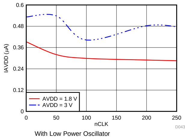
Figure 73. I_{AVDD} in High Precision Mode with nCLK
