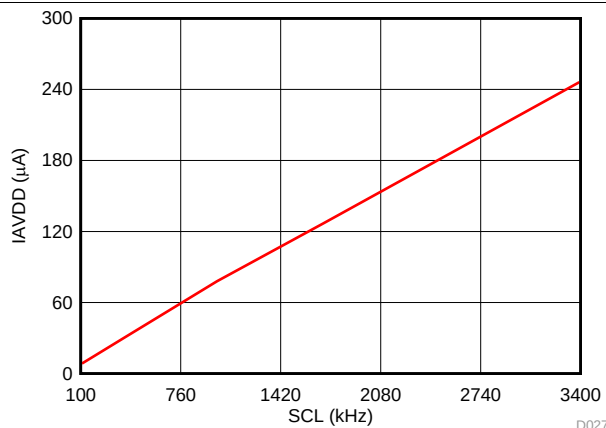
Figure 69. I_{AVDD} in Manual Mode with SCL
