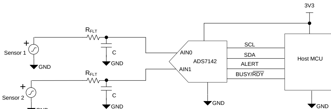
Figure 113. Sensor Monitor Circuit with ADS7142
