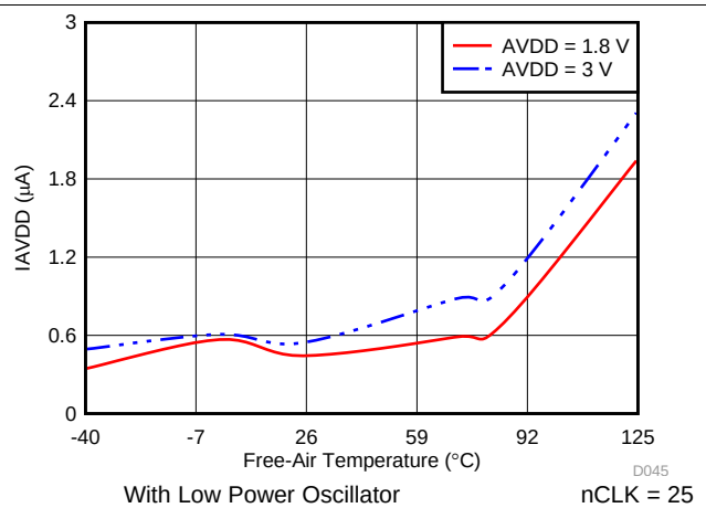
Figure 37. I_{AVDD} in High Precision Mode with Temperature
