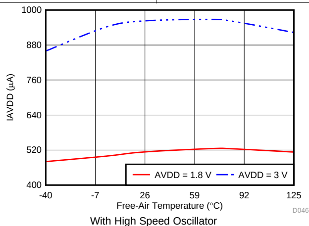
Figure 38. I_{AVDD} in High Precision Mode with Temperature
