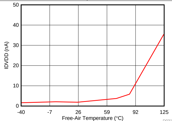
Figure 27. I_{DVDD} in Manual Mode with SCL
