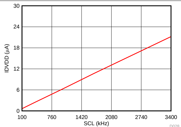
Figure 70. I_{DVDD} in Manual Mode with SCL
