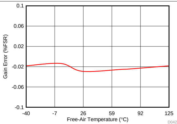
Figure 36. Gain Error in High Precision Mode with Temperature
