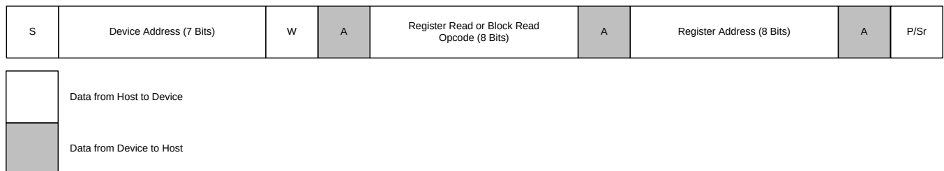
Figure 49. Setting Register Address for Reading Registers
