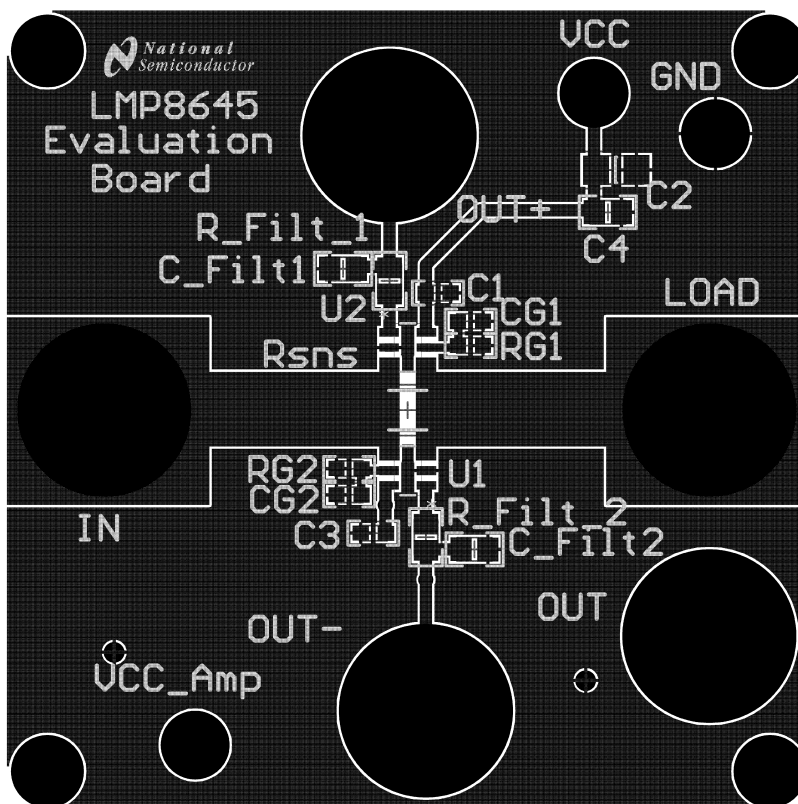
Figure 3. Top Layer
