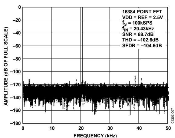
Figure 13. FFT Plot
