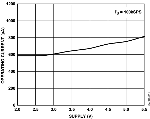
Figure 17. Operating Current vs. Supply
