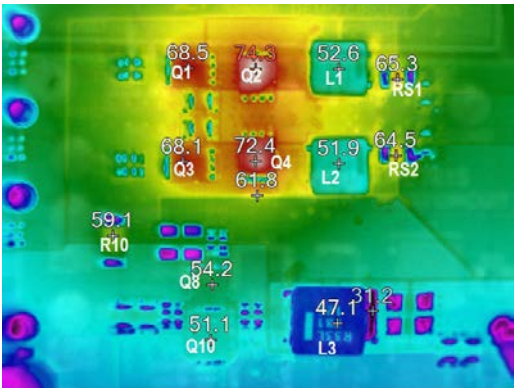
Figure 6. Thermal Image V_{IN} 12V, V_{o1} 5V at 8A, V_{o2} 3.3V at 8A, No Air Flow, T_A = 25^{\circ}C
