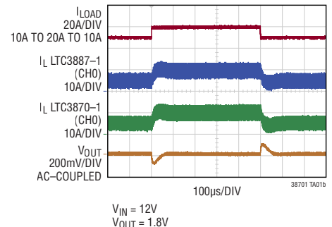
Load Transient Response of a 2-Phase Master (3887-1)/Slave (3870-1) Converter
