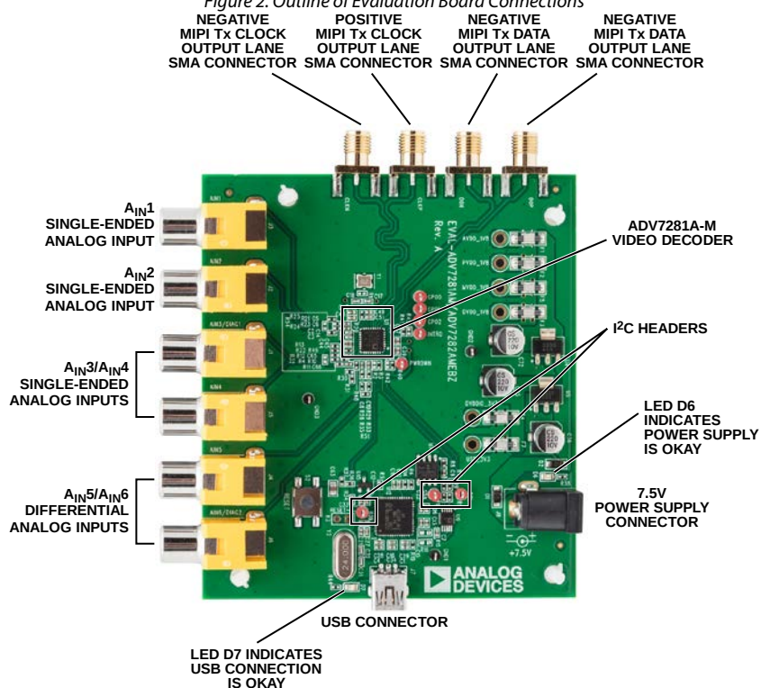
Figure 3. ADV7281A-M Evaluation Board
