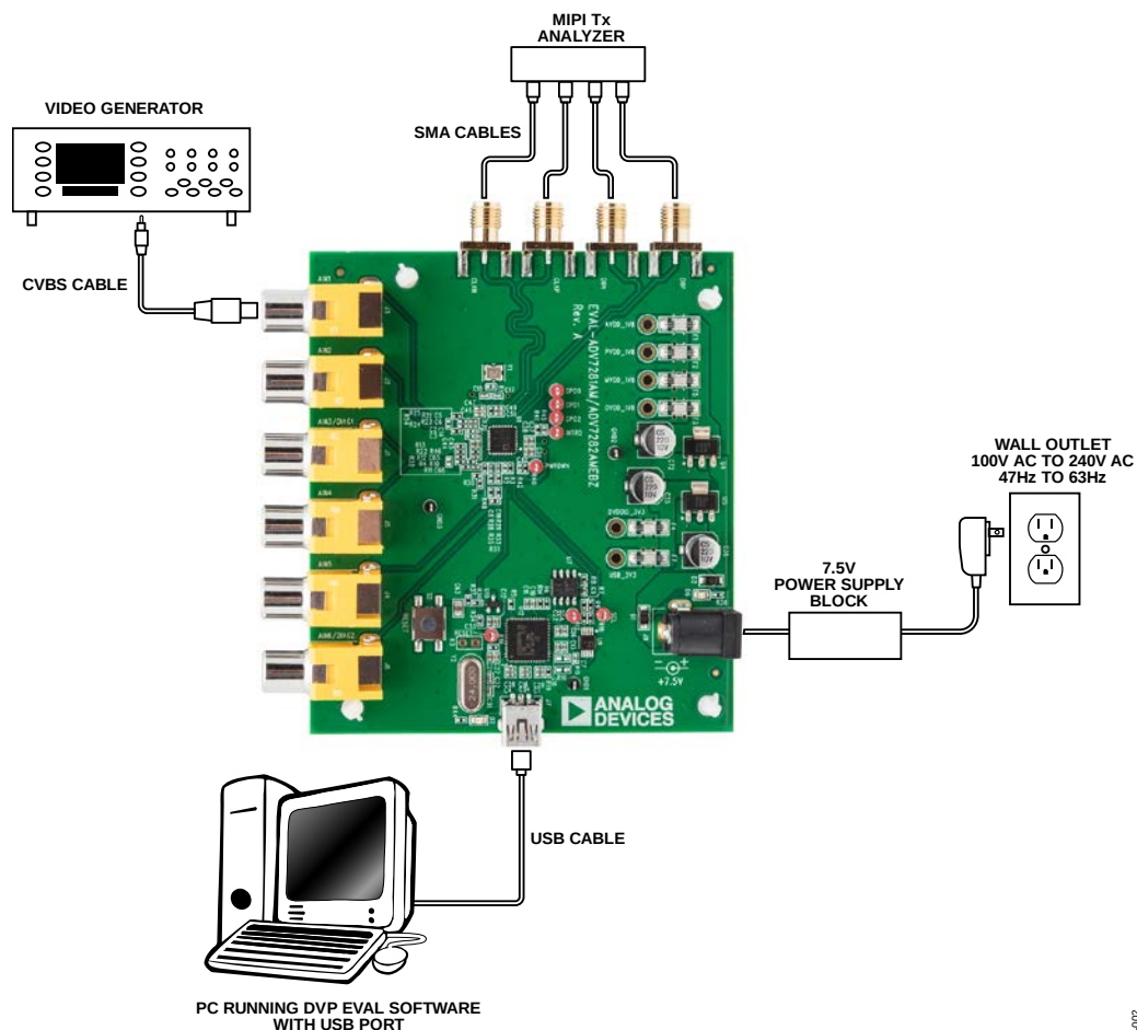
Figure 2. Outline of Evaluation Board Connections
