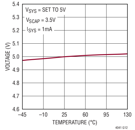
Backup Boost Output Voltage ( V_{SYS} ) vs Temperature
