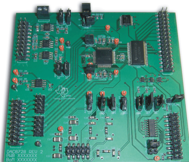
DAC8728EVM
