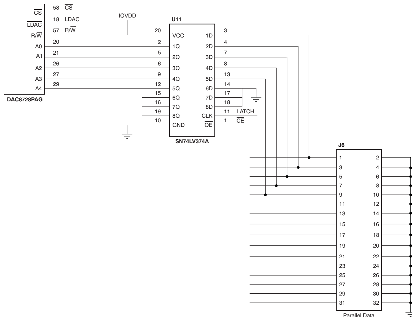
Figure 4. Shared 16-Bit Parallel Bus
