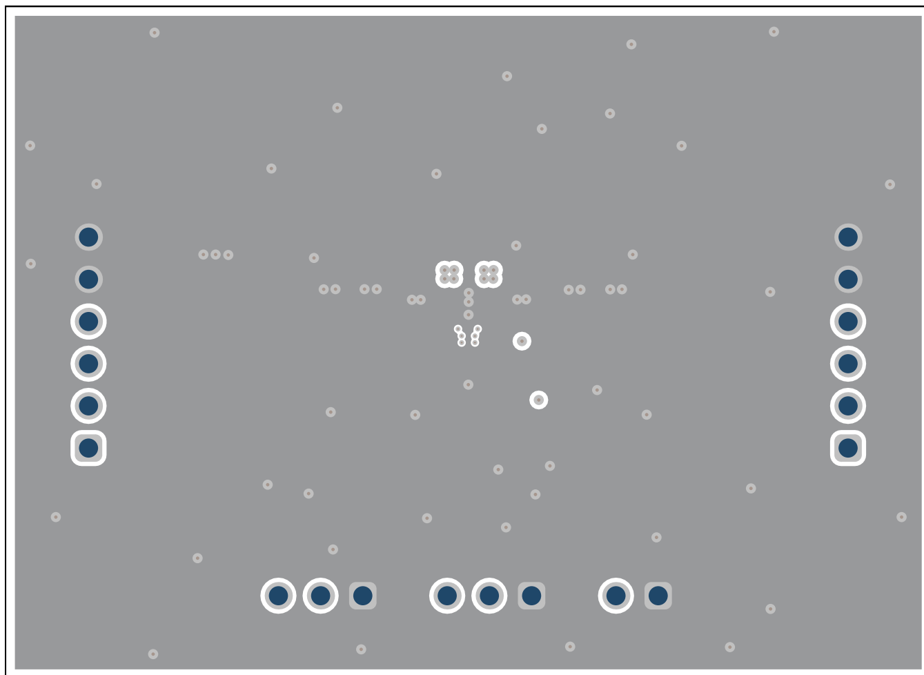
Figure 5. Signal Layer 2
