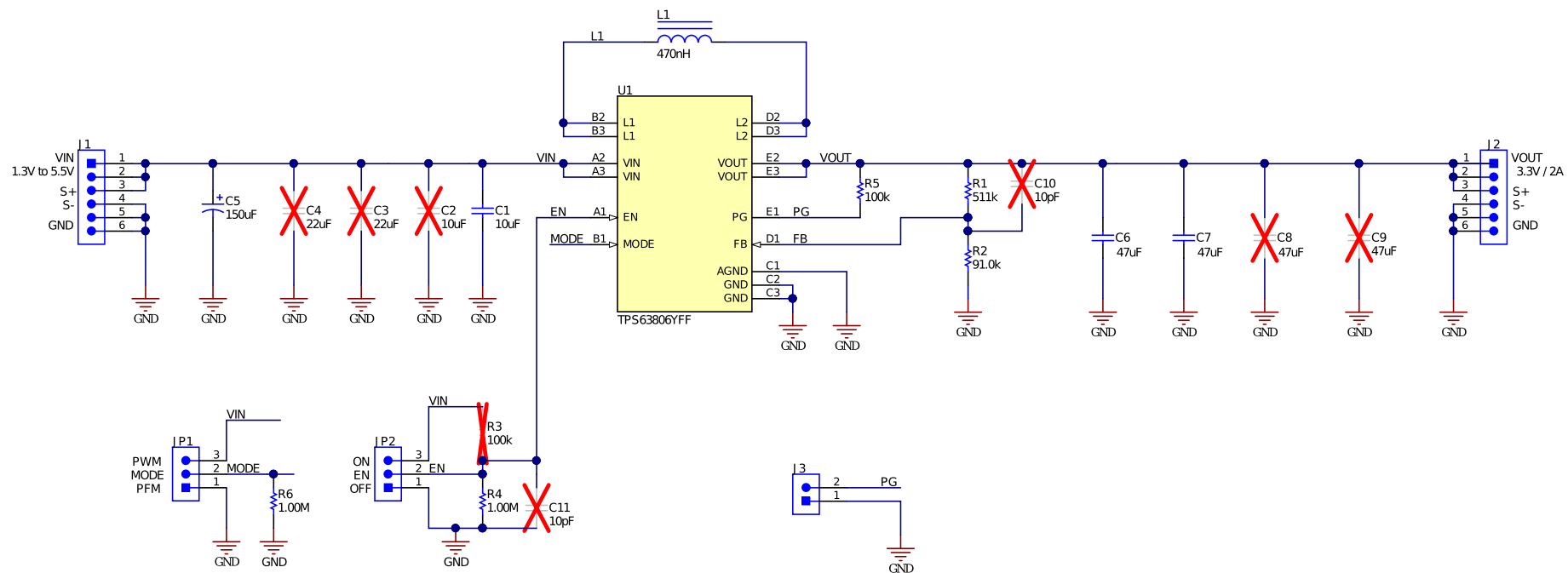
Figure 7. Schematic
