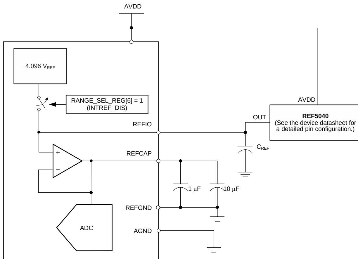
Figure 57. Device Connections for Using an External 4.096-V Reference
