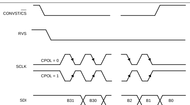
Figure 72. Standard SPI Timing Protocol (CPHA = 1, 32 SCLK Cycles)
