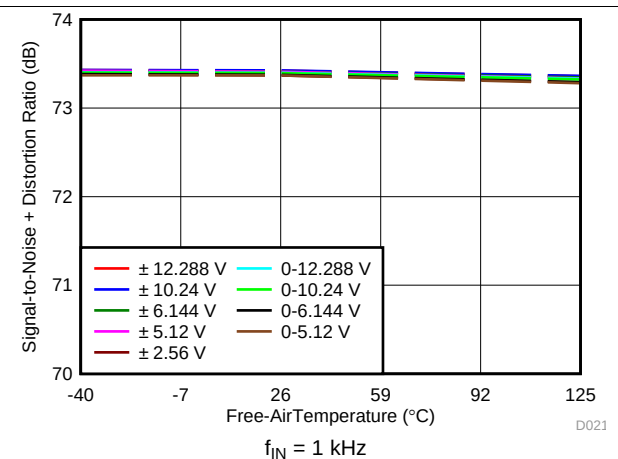
Figure 38. SINAD vs Temperature
