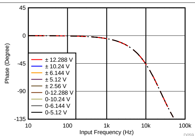
Figure 51. Second-Order LPF Phase Response
