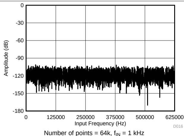
Figure 33. Typical FFT Plot (All Ranges) for the ADS8661
