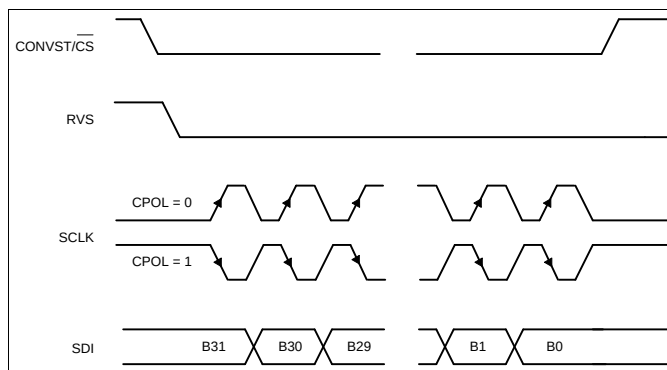
Figure 71. Standard SPI Timing Protocol (CPHA = 0, 32 SCLK Cycles)
