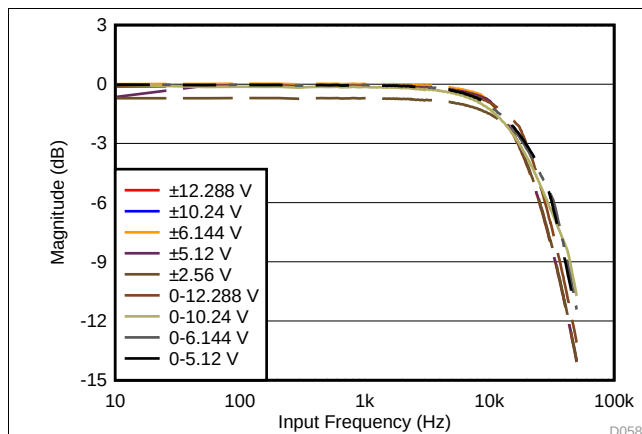
Figure 50. Second-Order LPF Magnitude Response
