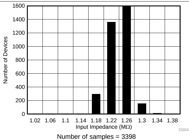
Figure 12. Typical Distribution of Input Impedance
