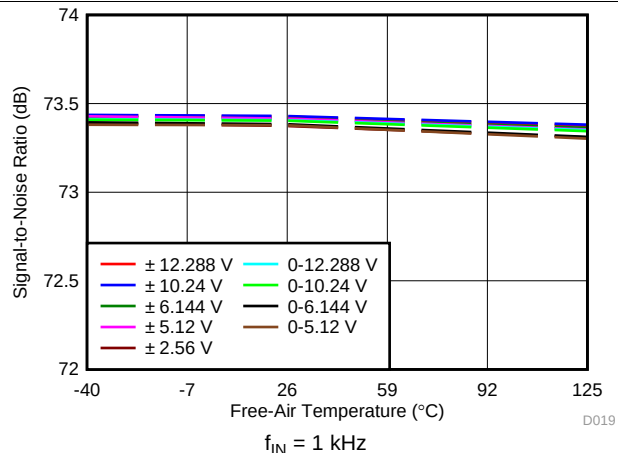
Figure 36. SNR vs Temperature
