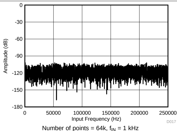
Figure 34. Typical FFT Plot (All Ranges) for the ADS8665
