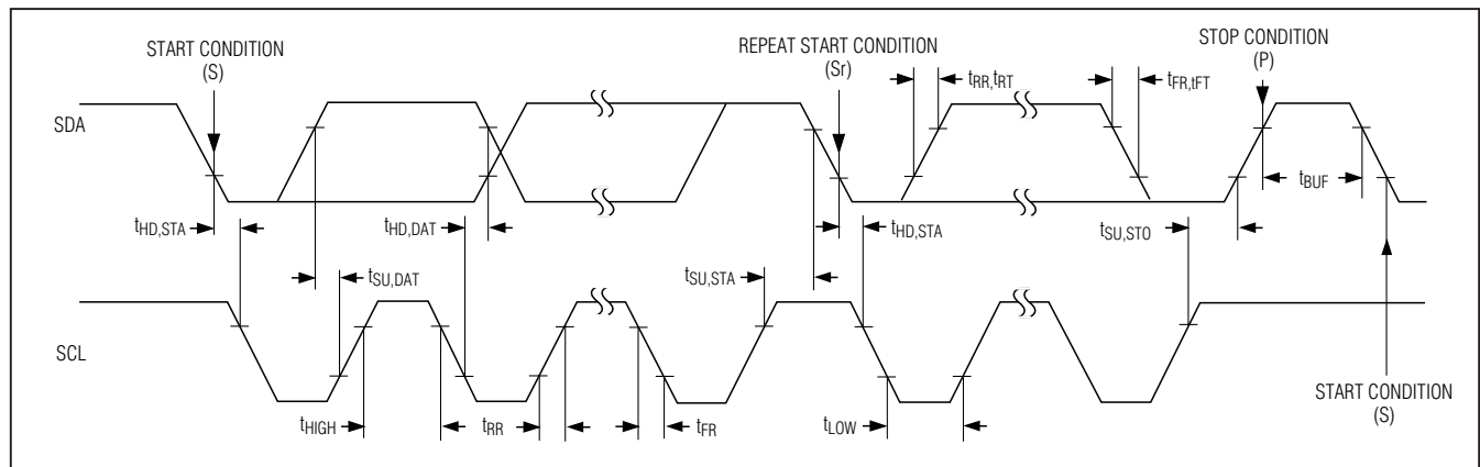
Figure 1. I²C Serial-Interface Timing
