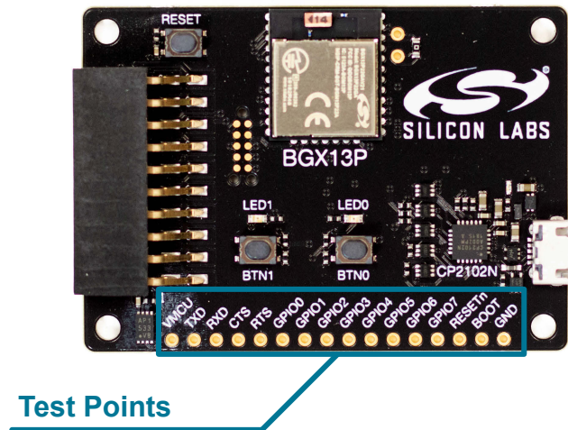
Figure 6.1. Test Points
