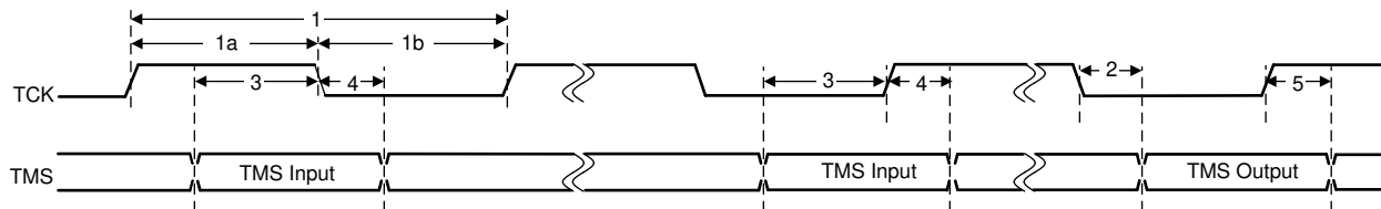
Figure 5-20. cJTAG Timing
