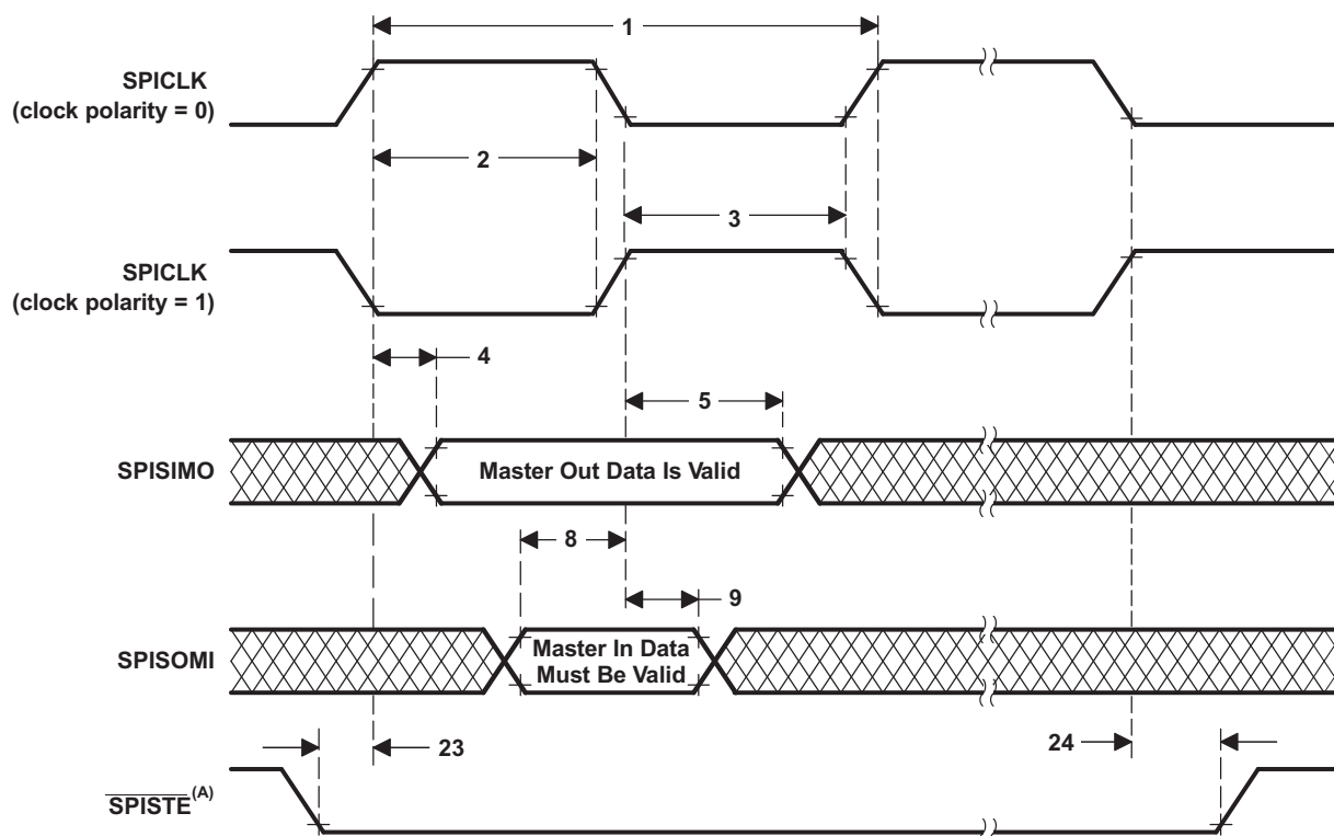
Figure 5-79. High-Speed SPI Master Mode External Timing (Clock Phase = 0)
