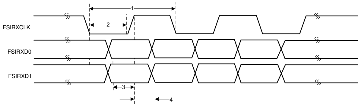
Figure 5-89. FSIRX Timings
