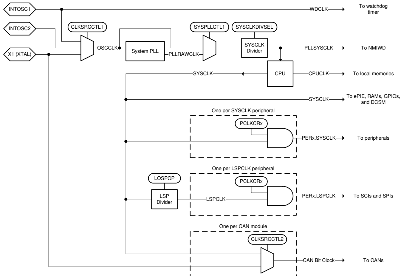
Figure 5-10. Clocking System
