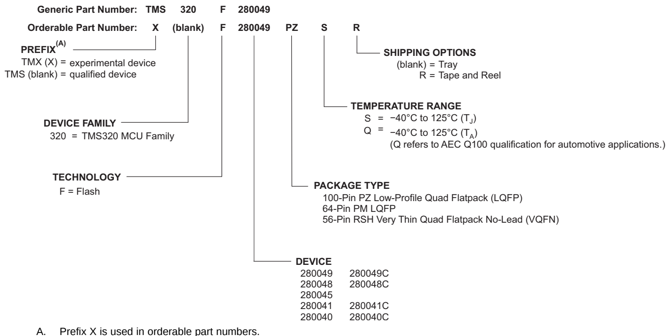
Figure 8-1. Device Nomenclature
