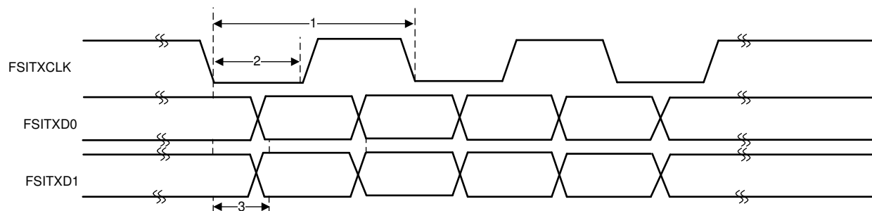
Figure 5-86. FSITX Timings
