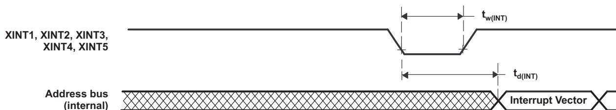
Figure 5-25. External Interrupt Timing
