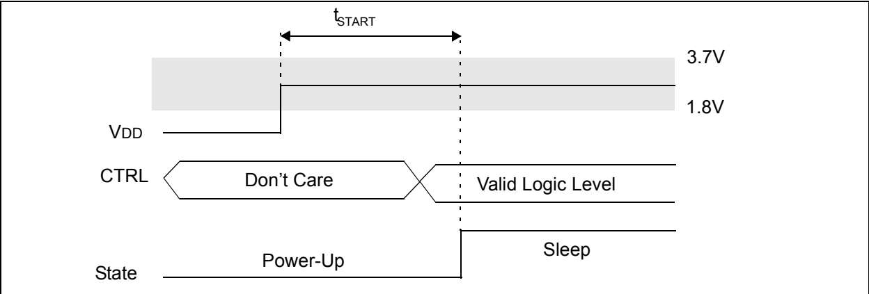
FIGURE 9-5: POWER-UP TIMING
