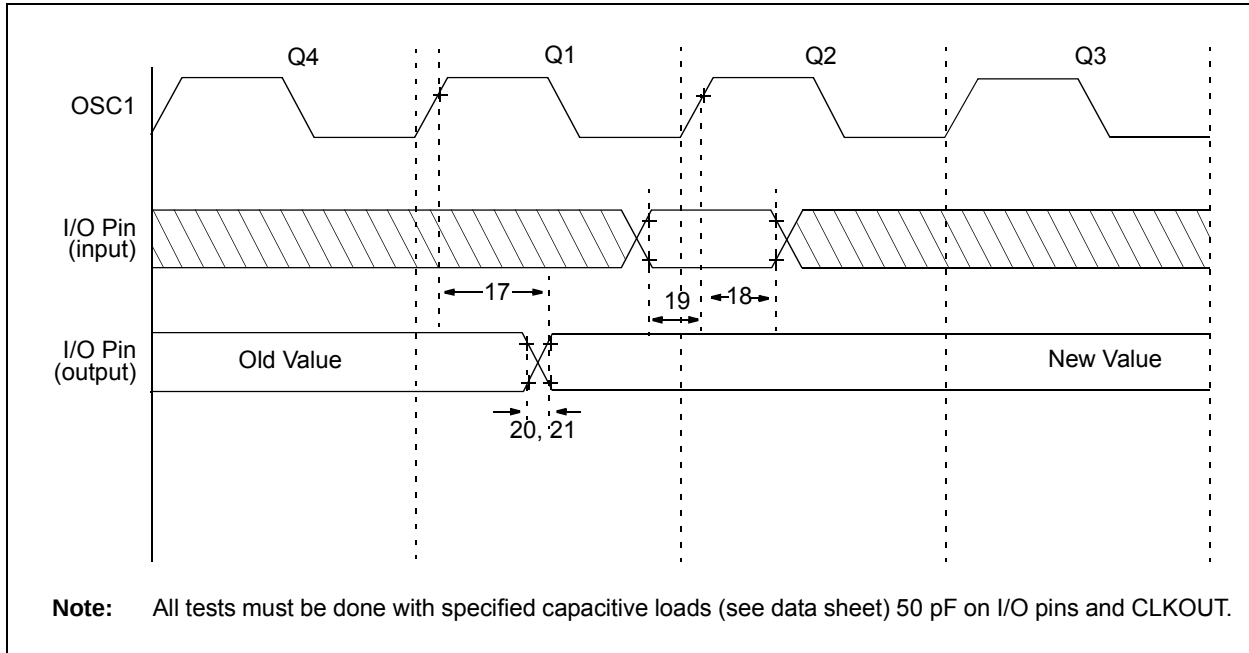
FIGURE 12-5: I/O TIMING
