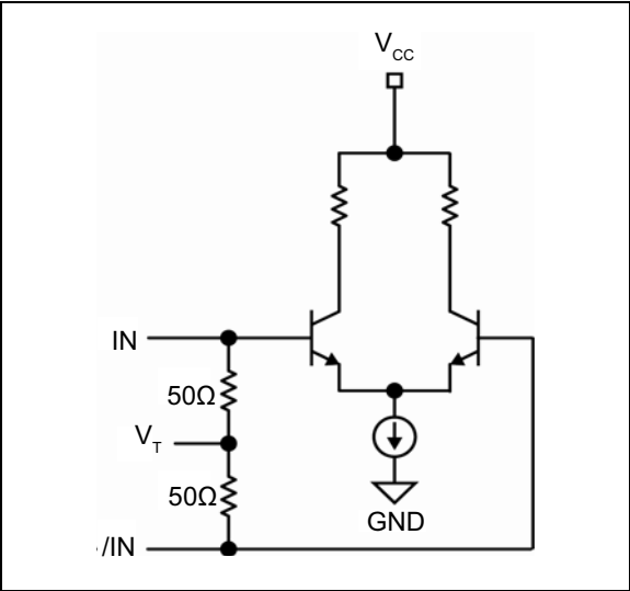
FIGURE 6-1: Input Stage.
