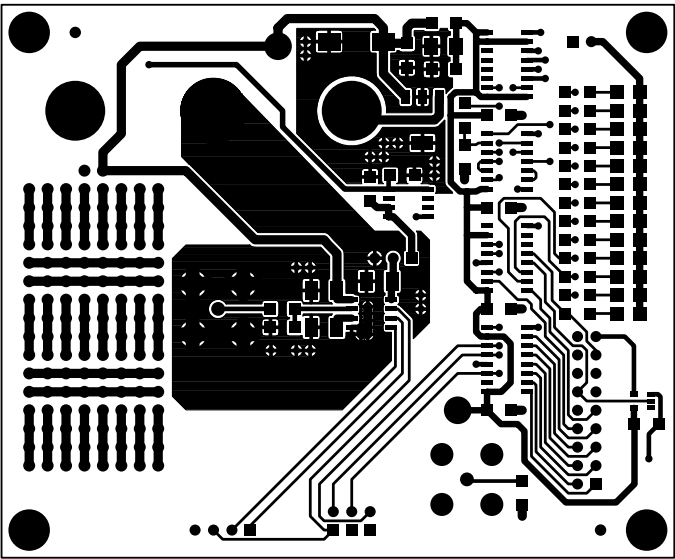
Component Side
