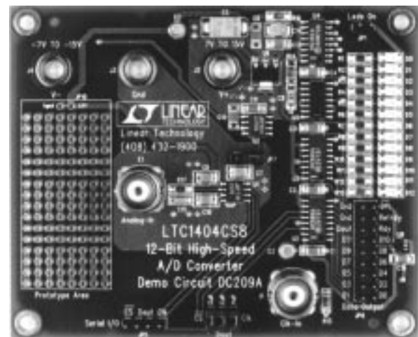
Board Photo
