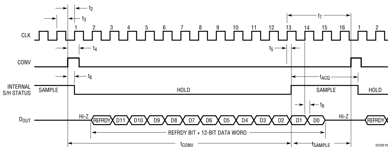
Figure 2. ADC Digital Timing Diagram (Timing Specifications Are Found in the LTC1404 Data Sheet)
