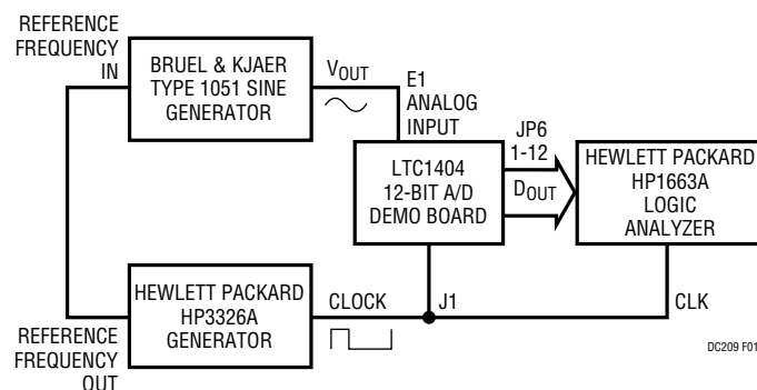
Figure 1. Typical Setup for LTC1404 Demo Board
