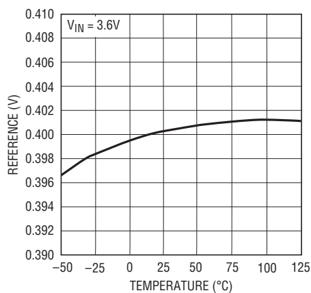
VLDO/Linear Regulator vs Temperature
