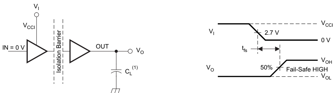
Figure 2. Failsafe Delay Time Test Circuit and Voltage Waveforms
