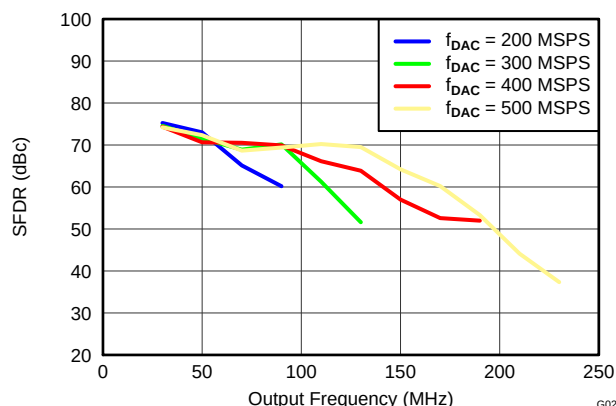
Figure 29. DAC3164 SFDR vs Output Frequency Over f_{DAC}
