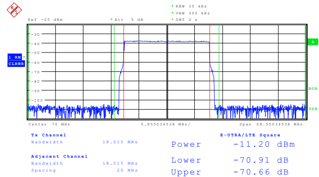
Figure 43. DAC3164 ACPR LTE 20-MHz FDD E-TM 1.1
