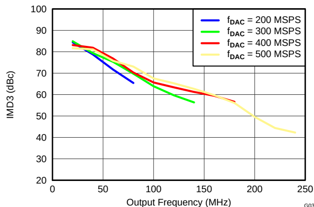
Figure 31. DAC3164 IMD3 vs Output Frequency Over f_{DAC}
