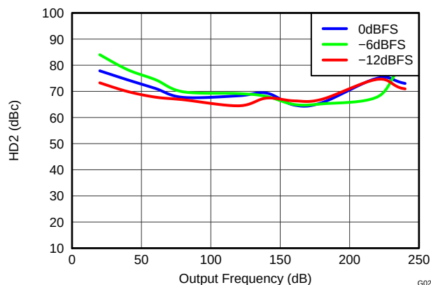
Figure 27. DAC3164 Second-Order Harmonic Distortion vs Output Frequency Over Input Scale
