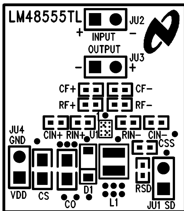
Figure 3. Silkscreen Top
