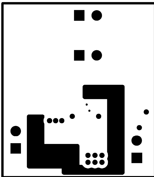
Figure 7. Bottom Layer
