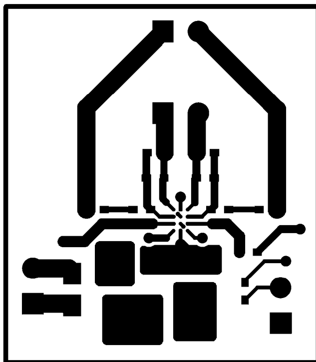
Figure 4. Top Layer
