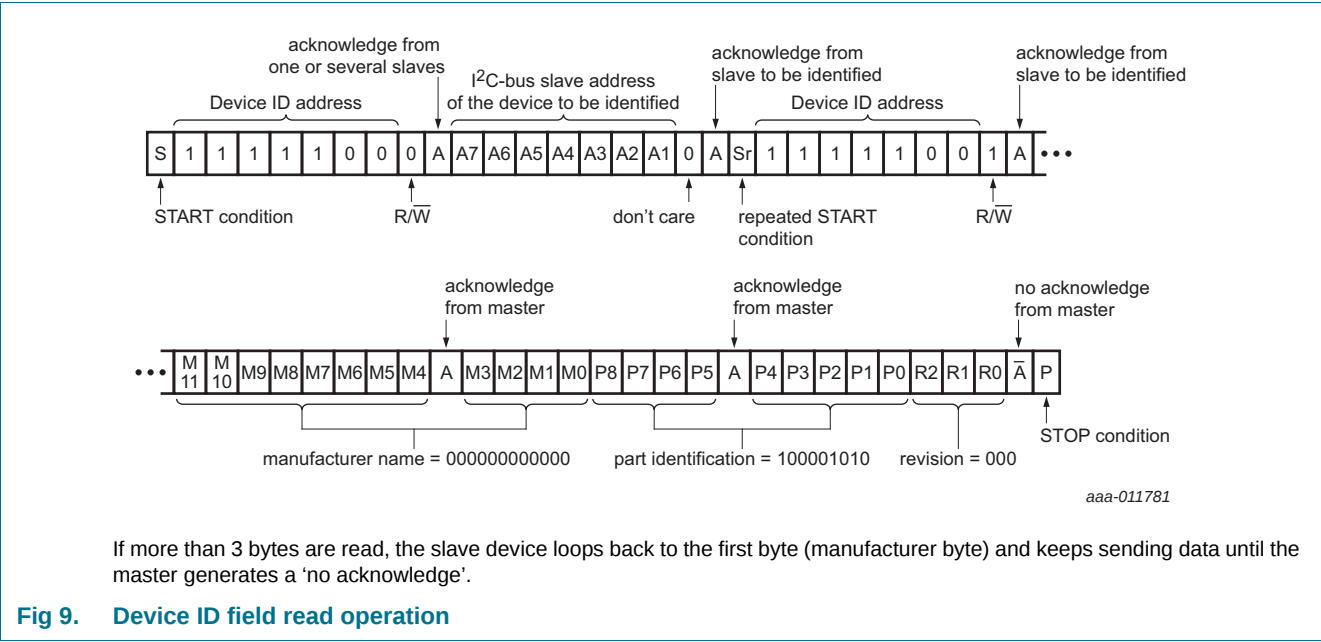
Fig 8. PCA9849 Device ID field
