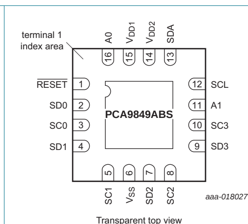
Fig 3. Pin configuration for HVQFN16
