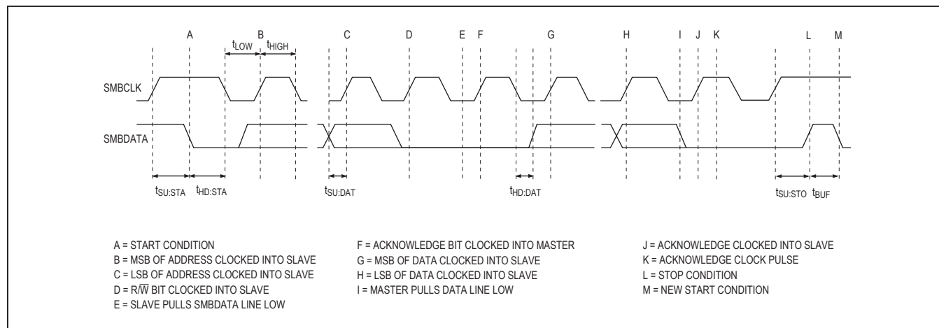
Figure 2. SMBus/I²C Write Timing Diagram
