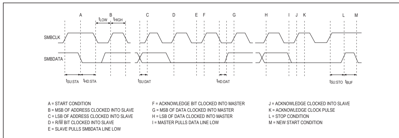
Figure 3. SMBus/I²C Read Timing Diagram
