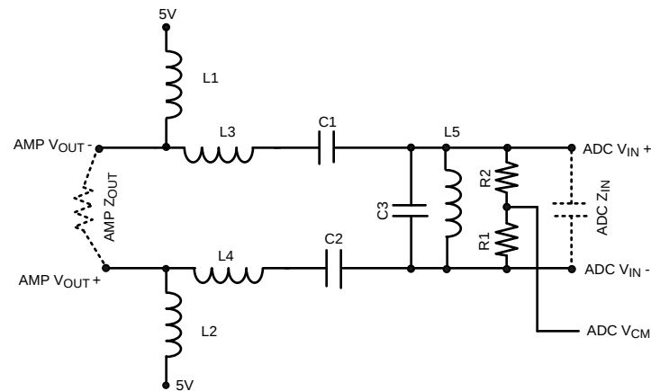
Figure 51. Sample Filter
