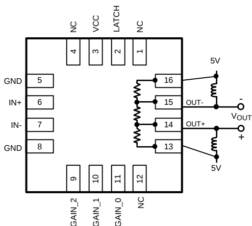
Figure 54. Using Low Gain Mode (200Ω Load)
