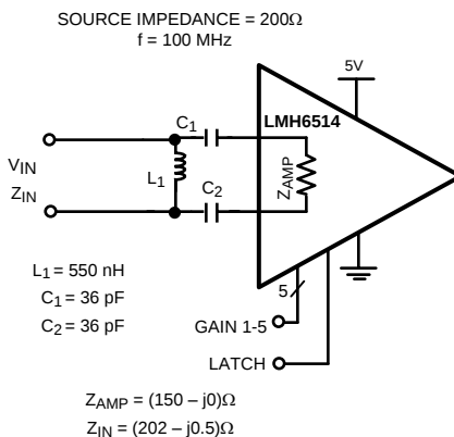
Figure 47. Differential 200Ω LC Conversion Circuit
