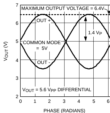
Figure 43. Output Voltage with Respect to the Output Common Mode
