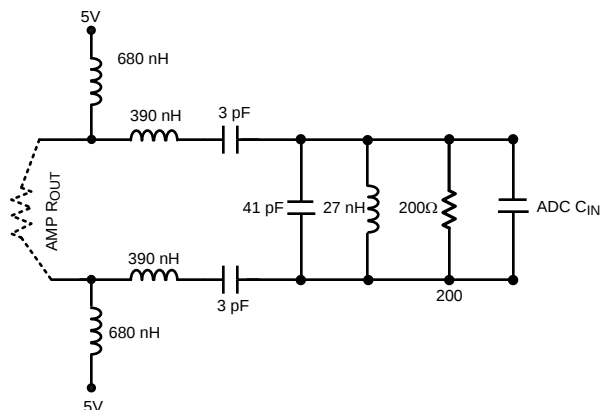
Figure 50. Bandpass Filter
