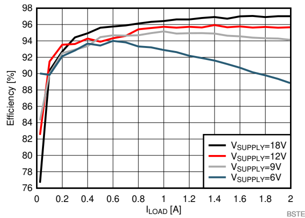
Figure 38. Efficiency
