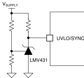
Figure 32. Inverted UVLO
