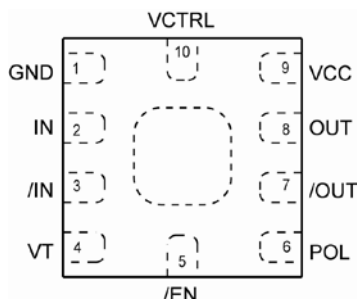
10-Pin MLF ® (2mm x 2mm) (MLF-10)
