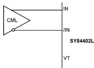
Figure 2d. DC-Coupled Input to CML
