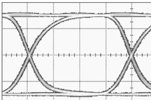
Electrical Eye Diagram at 4.25Gbps, PRBS 2^7-1 , R_L = 50\Omega
