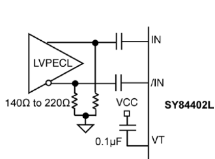
Figure 2a. AC-Coupled Input to LVPECL
