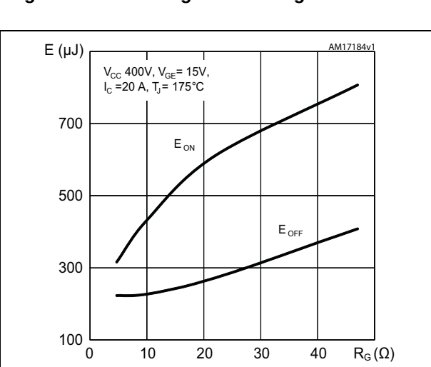
Figure 17. Switching losses vs. gate resistance
