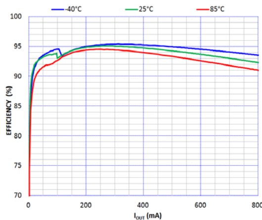
Figure 27. Efficiency vs Output Current vs Temperature PV_{IN} = 4.2\text{ V} , F_{sw} = 3.429\text{ MHz} , V_{OUT} = 3.3\text{ V}
