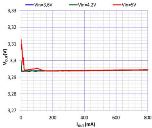
Figure 38. V_{OUT} Accuracy vs Output Current vs PV_{IN} @ 25^\circ\text{C} , F_{SW} = 3.429\text{ MHz} , V_{OUT} = 3.3\text{ V}
