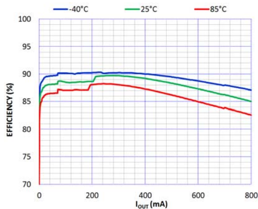
Figure 19. Efficiency vs Output Current vs Temperature PV_{IN} = 3.6\text{ V} , F_{SW} = 6\text{ MHz} , V_{OUT} = 1.8\text{ V}
