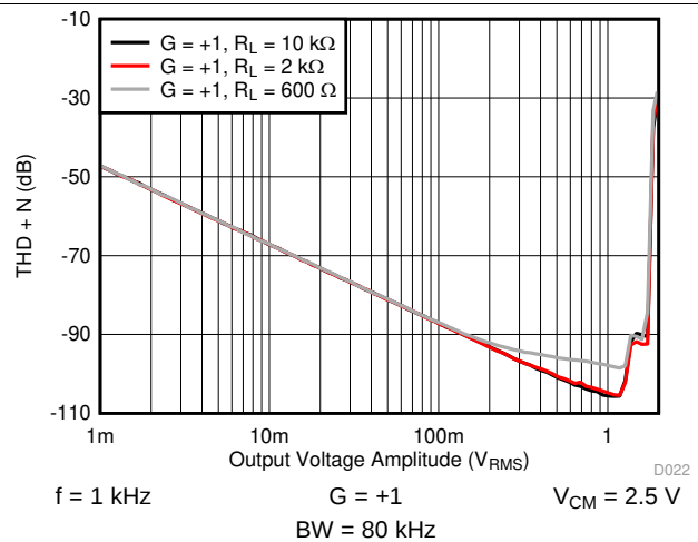
Figure 30. THD + N vs Amplitude
