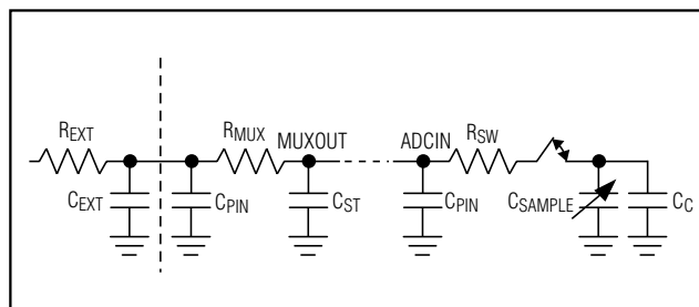
Figure 5. Analog Input, Unbuffered Mode ( \text{BUFF} = 0 )
