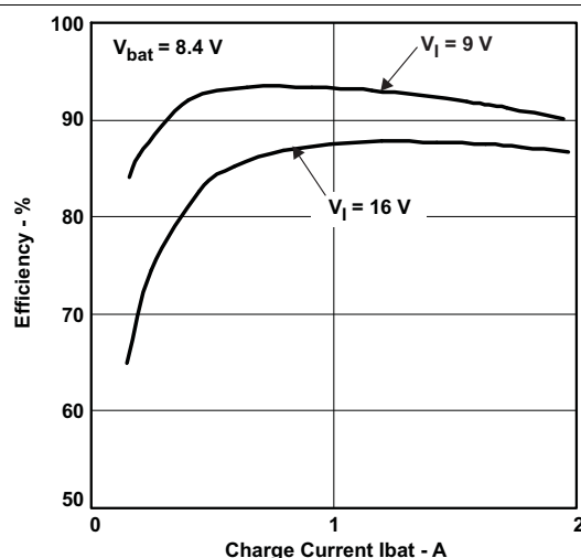
Figure 2. Efficiency 2-Cells
