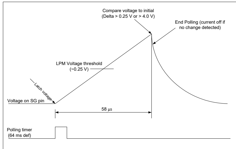
Figure 15. Low-power mode polling check
