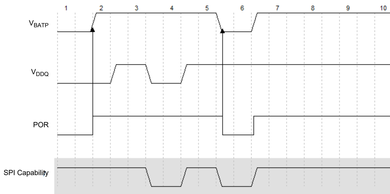
Figure 13. VBATP power up first
